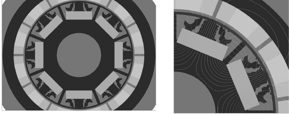
Figure 2: Final design of two-stage algorithm together with magnetic field lines. Figures taken from [13].
