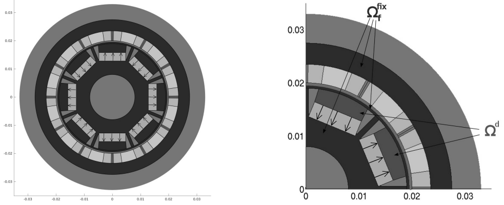
Figure 1: Left: Computational domain D representing electric motor with different sub-domains. Right: Zoom on upper right quarter (for a different rotor-to-stator constellation) with design region \Omega^d and fixed ferromagnetic set \Omega_f^{fix} . For a given design \Omega \subset \Omega^d , we have \overline{\Omega}_f = \overline{\Omega_f^{fix}} \cup \overline{\Omega} . Figures taken from [13].
